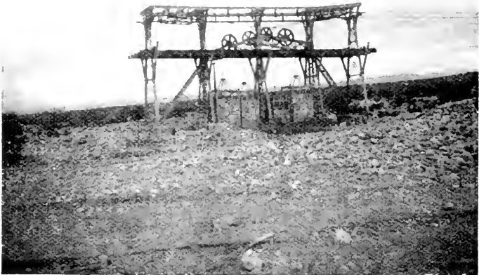
FAMATINA MINE—TENSION STATION OF AERIAL ROPE-WAY.
